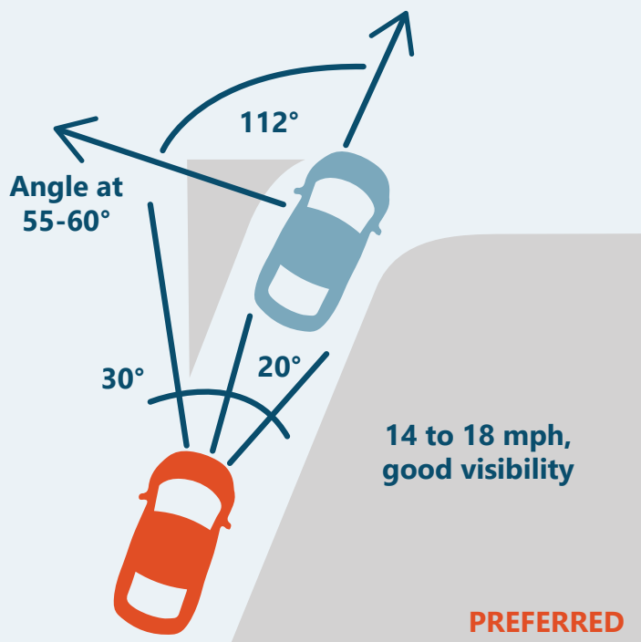
Figure 6 | Channelized Right Turn Lane
